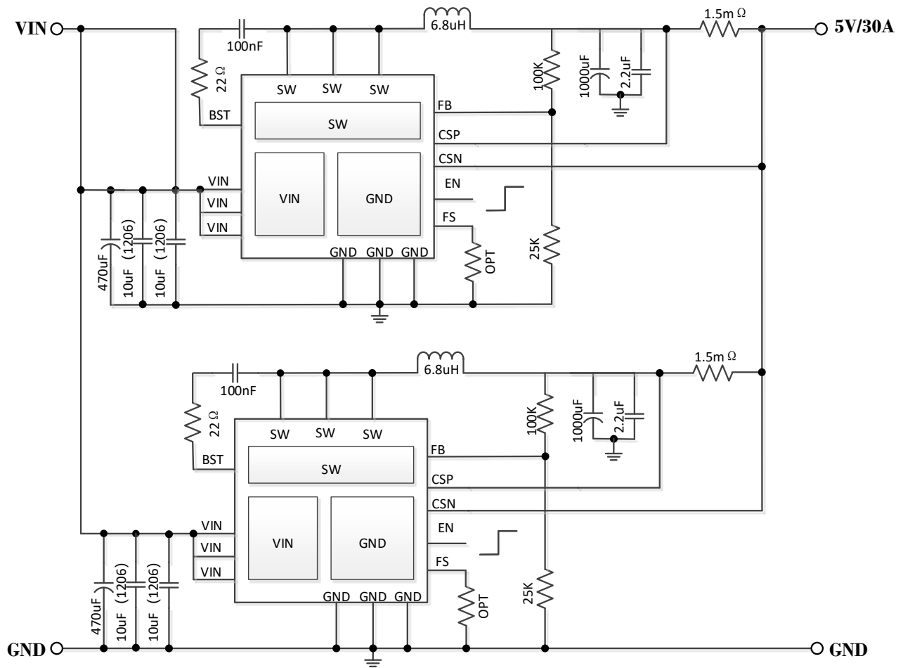
Dual Channel Power Supply
